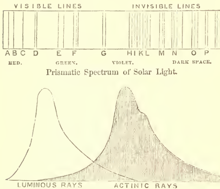
Curves representing the comparative intensity of the luminous and actinic rays in different parts of the solar spectrum.
